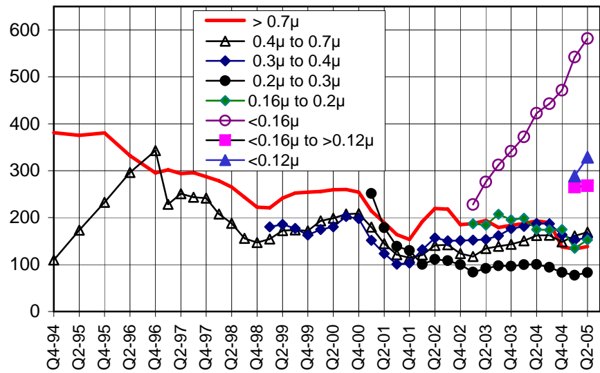
MOS 300 mm Wafers Utilization and Capacity
