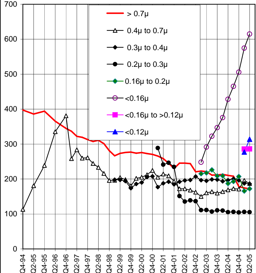
MOS Fab Capacity (wafer starts k/week) by Line Width, 8" equivalent
