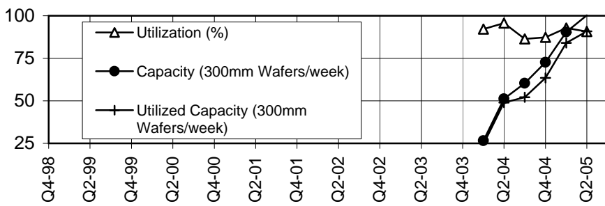
MOS 300 mm Wafers Utilization and Capacity
